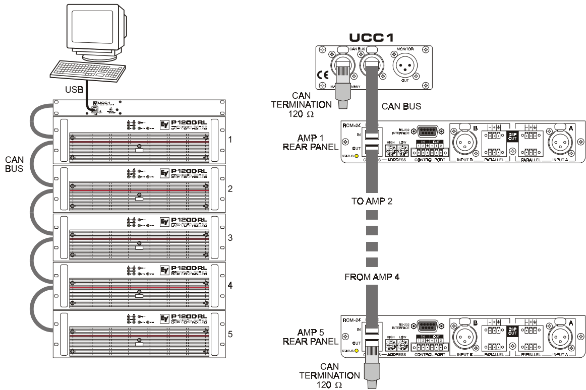
Fig 4: System set-up with 5 amps and a single UCC1 / PC being the first unit on the bus Terminators at the UCC1 (first unit) and at the amp No.5 (last unit on the bus)
