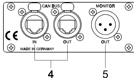
Fig 2: UCC1 rear view
