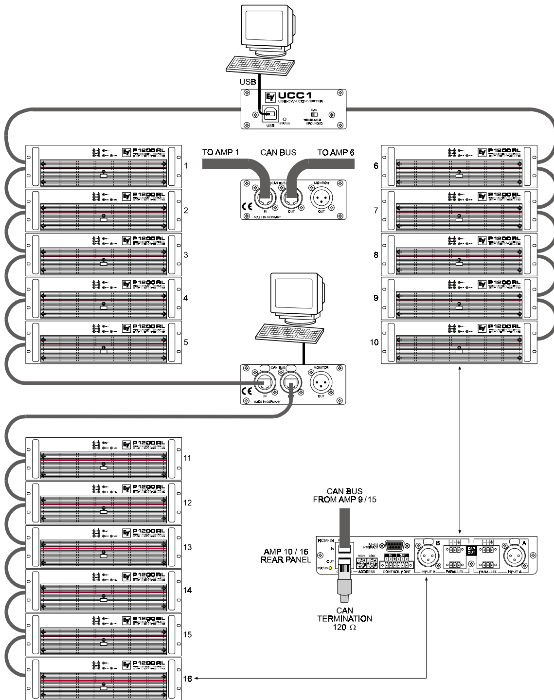
Fig 6: System with several racks and several UCC1 / PCs UCC1 anywhere on the CAN-bus Terminators at amp No. 10 (first unit) and amp No. 16 (last unit on the bus)
