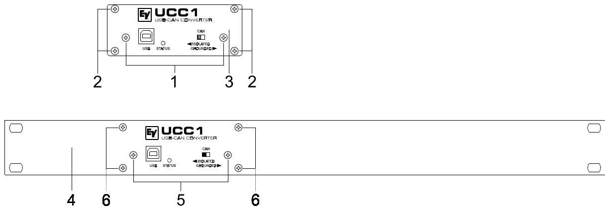
Fig. 3: Exchanging UCC1 front panels
