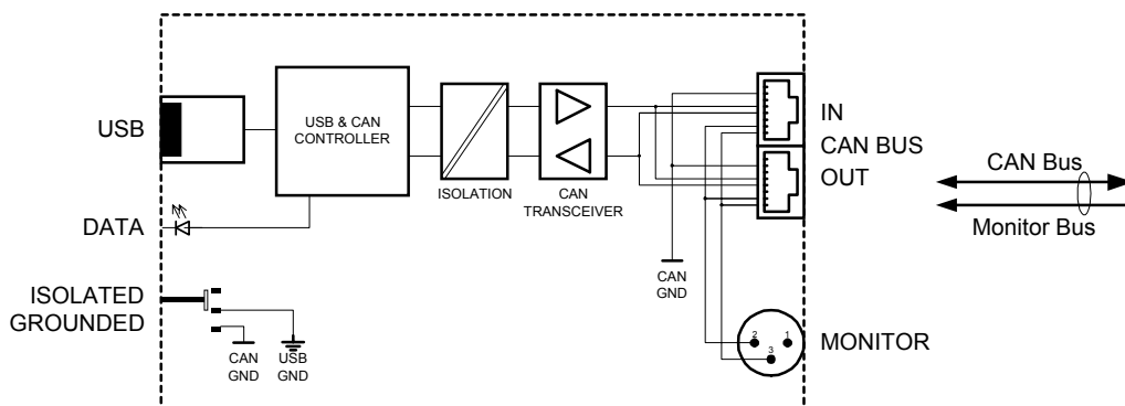
Fig. 7: UCC1 Block Diagram
