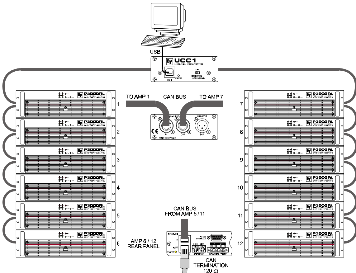
Fig 5: System set-up with 2 racks and a single UCC1 / PC in the middle Terminators at amp No. 6 (first unit) and amp No. 12 (last unit on the bus)
