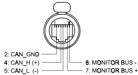
Fig. 8: CAN BUS IN / OUT connector pin-assignment
