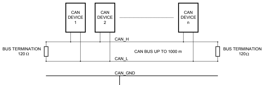
Fig. 9: Bus-topology of the CAN-bus
