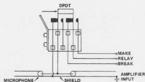
FIGURE 2 - Wiring Diagram
