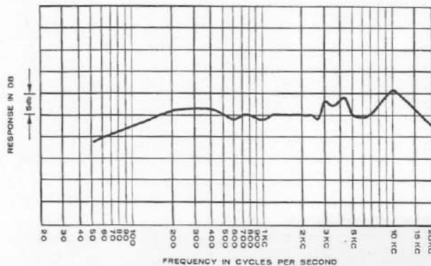
Fig. 1-Frequency Response
