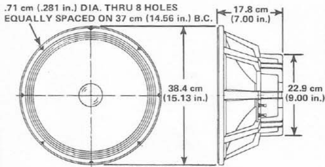
FIGURE 1 - Dimensions
