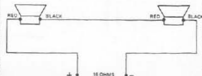
FIGURE 12 Connection of 2 EVM-15L Speakers in Series
