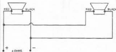
FIGURE 11 Connection of 2 EVM-15L Speakers in Parallel
