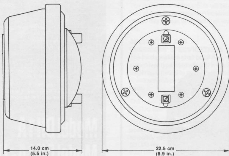
FIGURE 2 Dimensions
