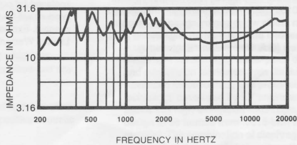
FIGURE 9 Impedance Response HP9040 Horn, 16-Ohm Driver
