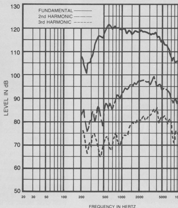
FIGURE 5 Distortion Response, HP9040 Horn, 10 Watts/1 Meter
