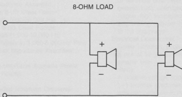
FIGURE 8 Electrical Connections
