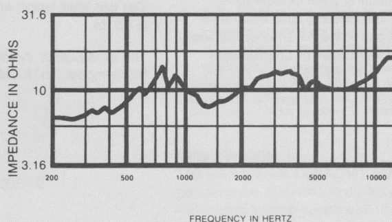
FIGURE 7 Impedance Response — HP9040 Horn
