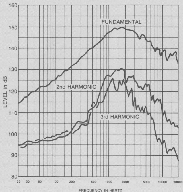
FIGURE 4 Distortion Response — 2-Inch Plane-Wave Tube, 8 Watts Input
