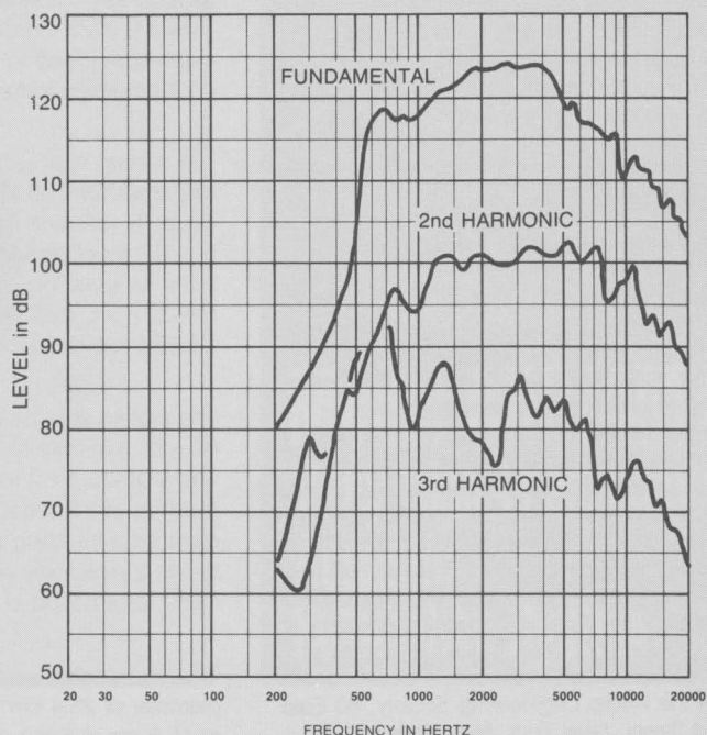
FIGURE 5 Distortion Response — HP64 Horn 8 Watts/1 Meter
