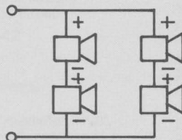
FIGURE 8 Electrical Connections
