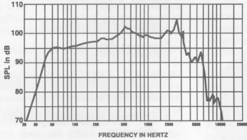
FIGURE 1 — Axial Response in Typical Enclosure (2.0 ft³), 1 Watt/1 Meter
