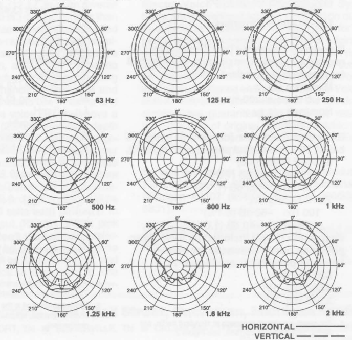
FIGURE 9 — Polar Response
