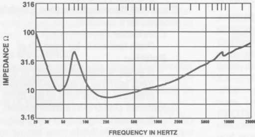
FIGURE 4 — Impedance in Typical Enclosure (2.0 ft³)
