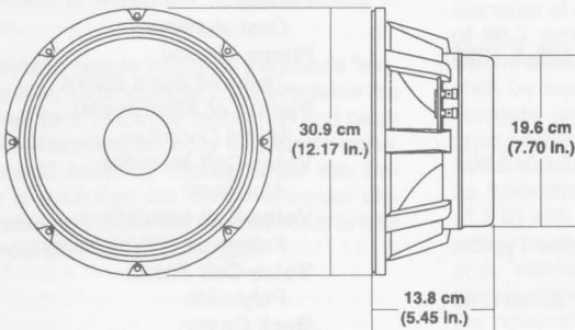
FIGURE 5 — Dimensions
