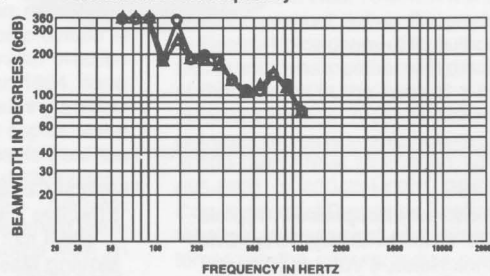
FIGURE 7 — Beamwidth vs. Frequency
