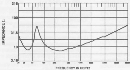
FIGURE 4 — Impedance in Typical Enclosure
